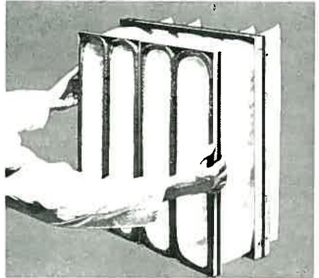
2-ADG Front filter media withdraw type
