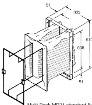
Multi-Peak MP21 standard flow overall depth 570
